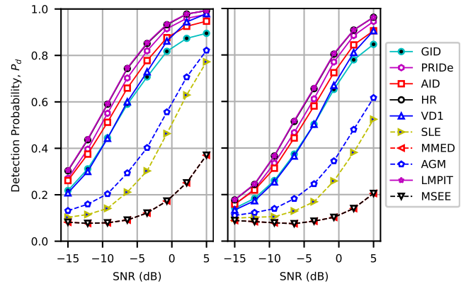
Fig. 2: Detection probability, P_d , for the standard parameter set, over targeted SNR varying from -15 to 5 dB for SNR Model 1 (left) and Model 2 (right).
