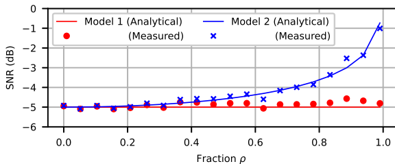
Fig. 1: Analytical and simulated SNR values for both models versus \rho .
