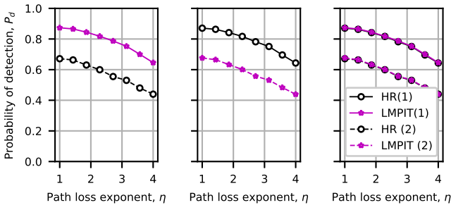
Fig. 4: SNR Model mismatch comparison for LMPIT and HR detectors, using SNR Models 1 and 2 respectively, on the left, 2 and 1 on center, and all models on the right, under standard simulation parameter set, for varying \eta .
