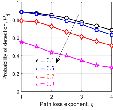
Fig. 8: P_d versus \eta for different \epsilon .
