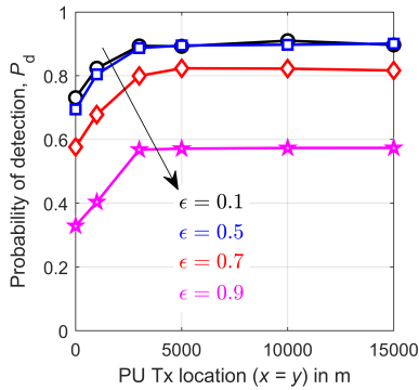
Fig. 9: P_d versus (x, y = x) for different \epsilon .
