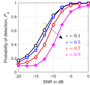
Fig. 6: P_d versus SNR for different \epsilon .
