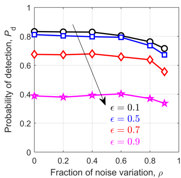
Fig. 10: P_d versus \rho for different \epsilon .
