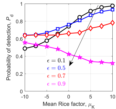
Fig. 7: P_d versus \mu_K for different \epsilon .
