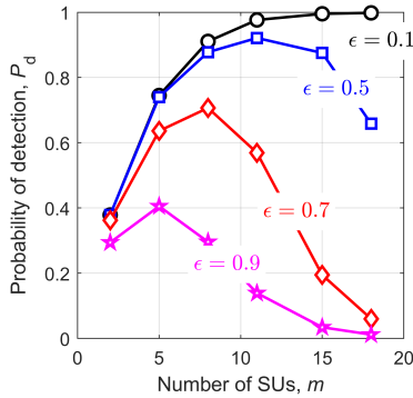
Fig. 4: P_d versus m for different \epsilon .
