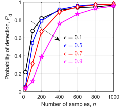
Fig. 5: P_d versus n for different \epsilon .
