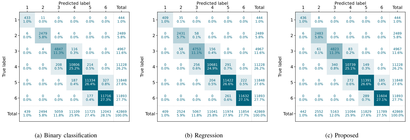
Fig. 3: Confusion matrices of the MF selection using the three ML-based strategies over the test set.
