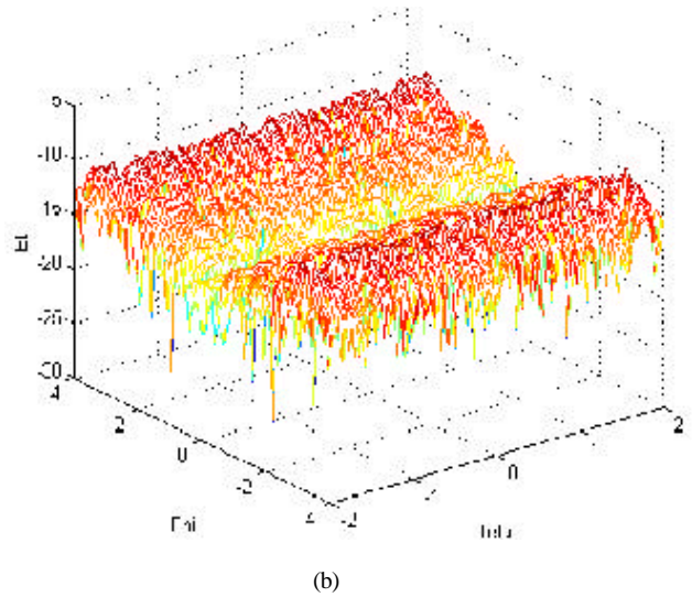
Fig. 4. Radiation Pattern as function of Phi and Theta for the microstrip planar antenna array, (a) (8x8) elements for \epsilon_r=16 and (b) (15x15) elements for \epsilon_r=4.4 .
