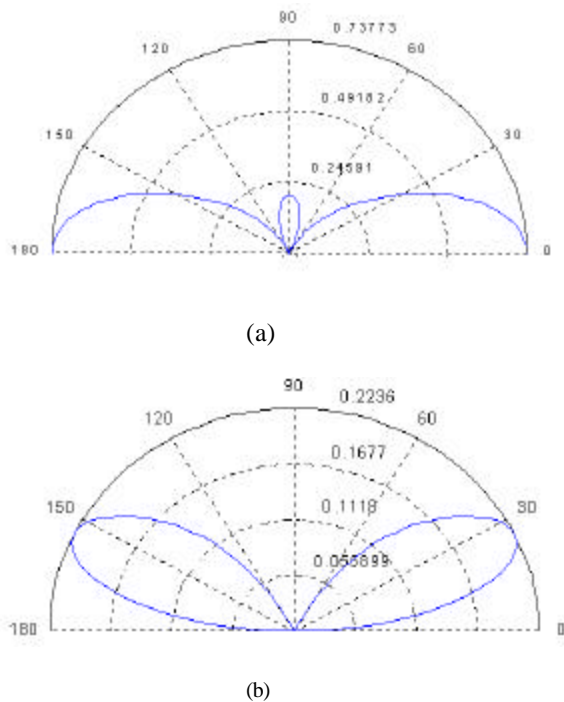
Fig. 4. Radiation Pattern as function of Phi and Theta for the microstrip planar antenna array, (a) (8x8) elements for \epsilon_r=16 and (b) (15x15) elements for \epsilon_r=4.4 .
