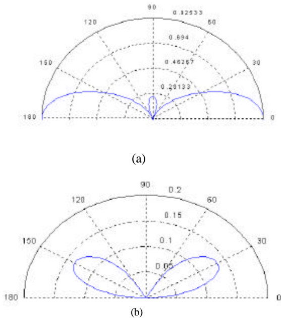
Fig. 2. Radiation Pattern field for the microstrip antenna of five elements, (a) to the E-plane and (b) to the H-plane.
