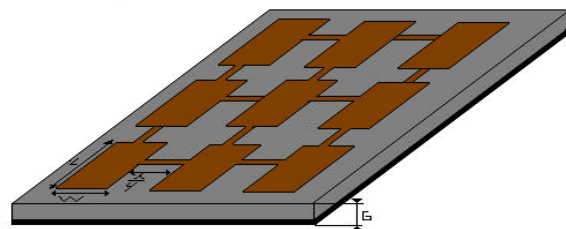
Fig. 1. Planar microstrip array of 3x3 elements.
