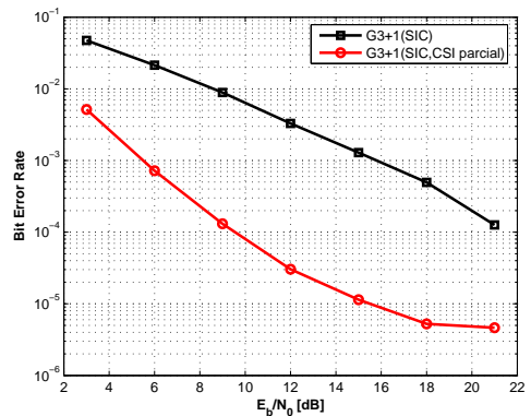
Fig. 7. Result for the second possible solution: partial CSI at transmitter side.
