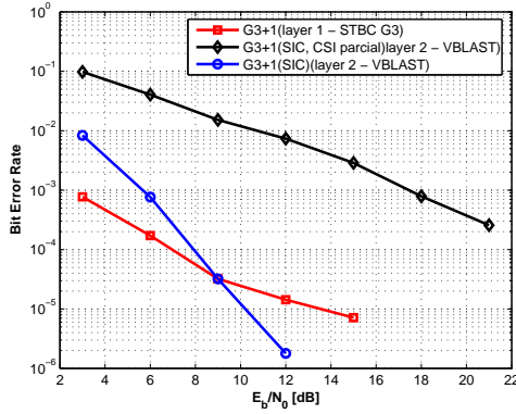
Fig. 8. Result per layer for the second possible solution: partial CSI at transmitter side.
