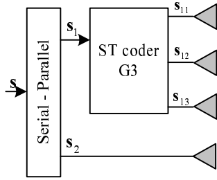
Fig. 2. Architecture of the HMTS G3+1 transmitter
