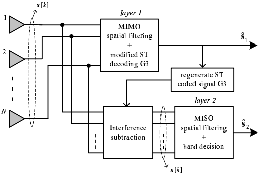
Fig. 3. Architecture of the HMTS G3+1 receiver, considering modified SIC as IC algorithm.
