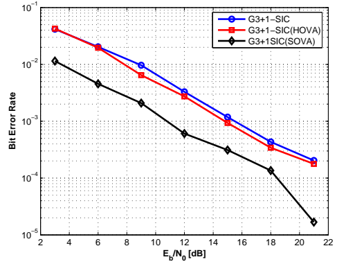
Fig. 5. Result for the first possible solution: channel coding.
