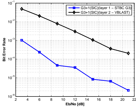
Fig. 4. Comparison of BER performance for the layers of the HMTS G3+1.
