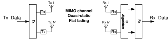
Fig. 1. MIMO schemes general structure.
