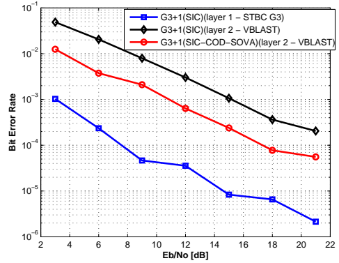
Fig. 6. Result per layer for the first possible solution: channel coding.
