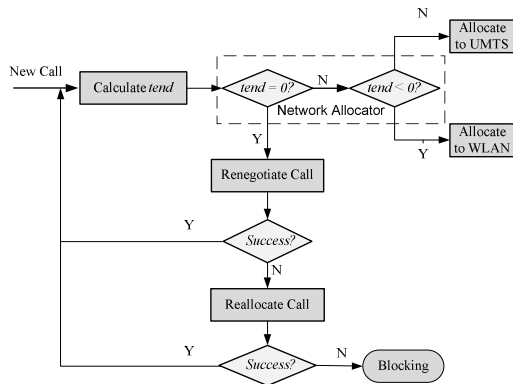
Fig. 1. Joint multi-radio resource management algorithm
