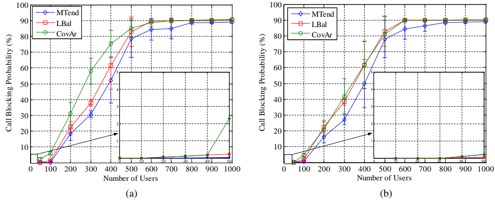
Fig. 2. Call blocking probability for real-time traffic, without (a) and with (b) call renegotiation
