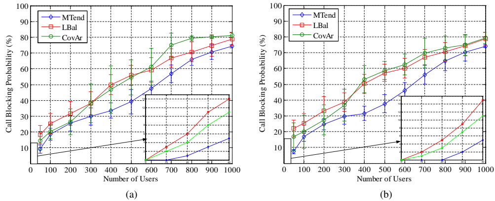
Fig. 3. Call blocking probability for real-time and non-real-time traffic, without (a) and with (b) call renegotiation
